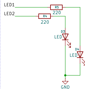
LEDS
